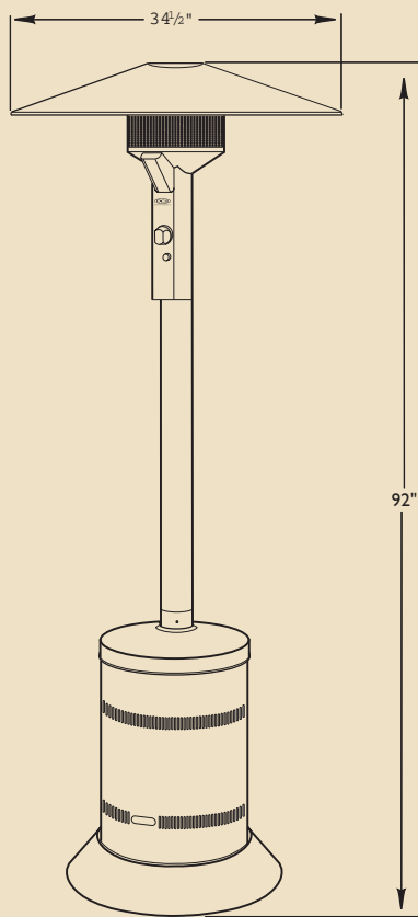
DCS PH1 Freestanding Model
